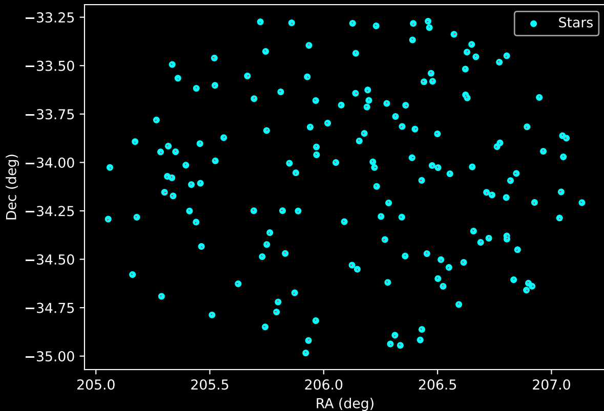
GALAH DR4 Field: [3728] Proper Motion Vectors for Gaia Star Field (n= 150)
