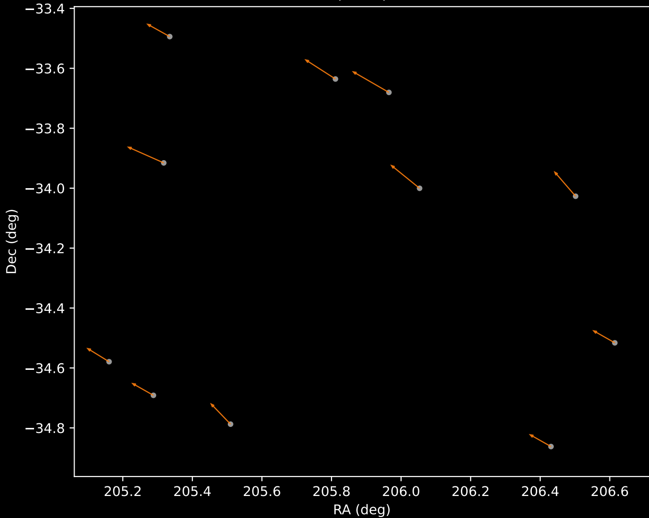
GALAH DR4 Cluster 2 Proper Motion Vectors (n=11)
