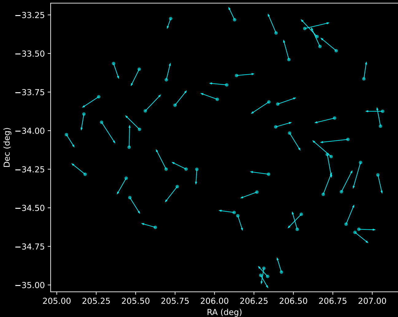
GALAH DR4 Noise Stream Proper Motion Vectors (n=58)
