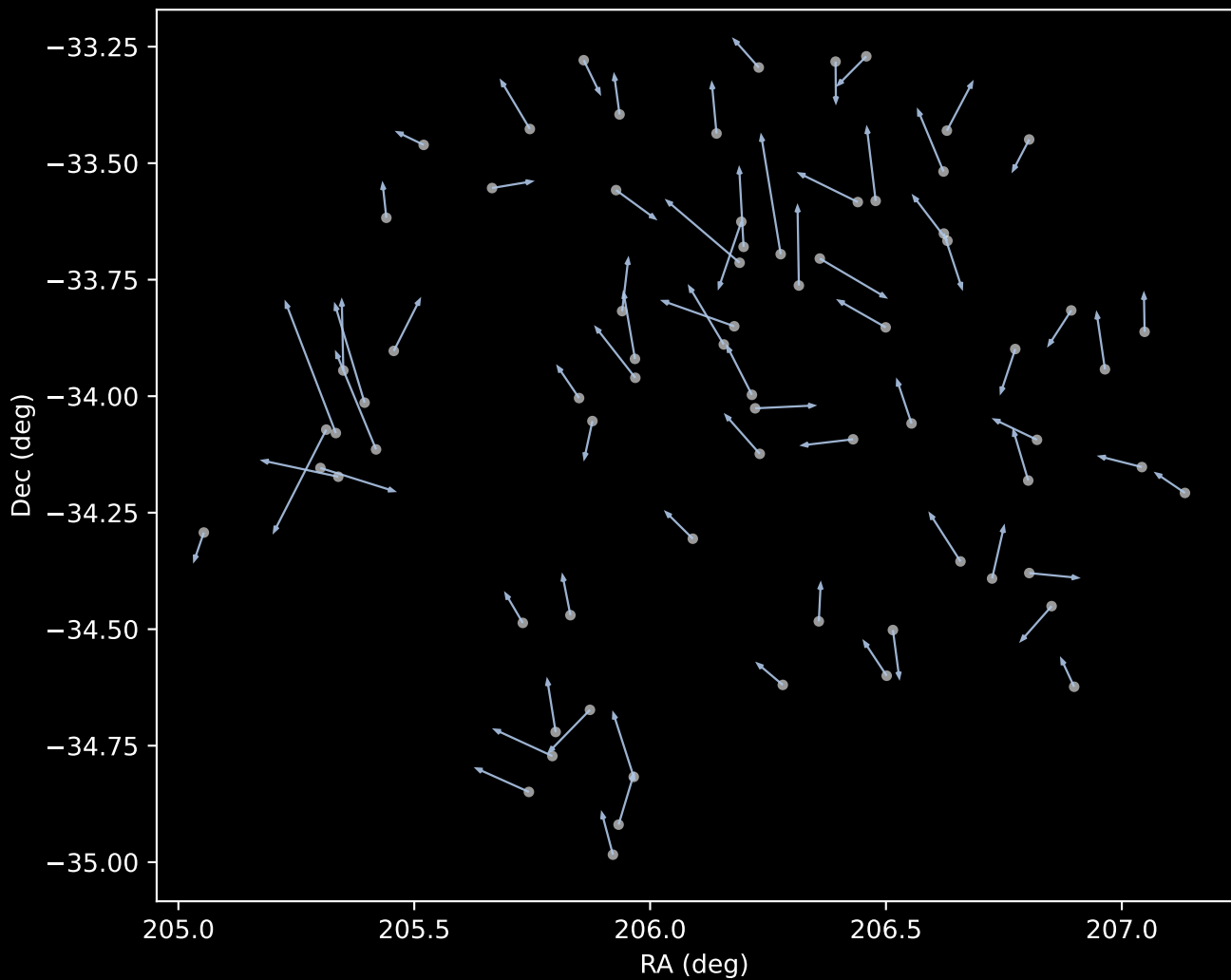
GALAH DR4 Cluster 1 Proper Motion Vectors (n=73)
