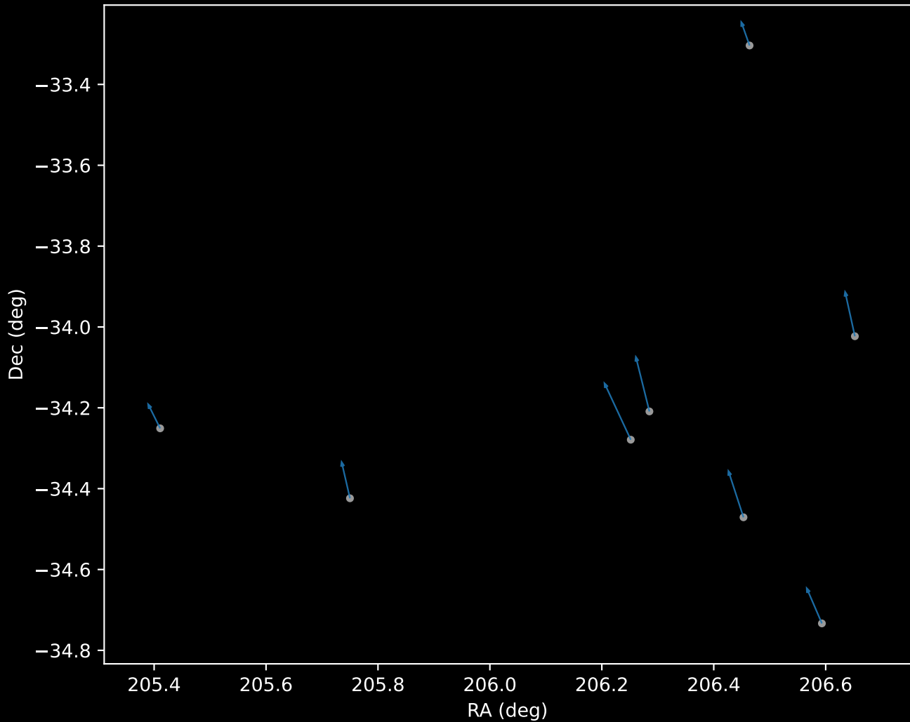
GALAH DR4 Cluster 0 Proper Motion Vectors (n=8)
