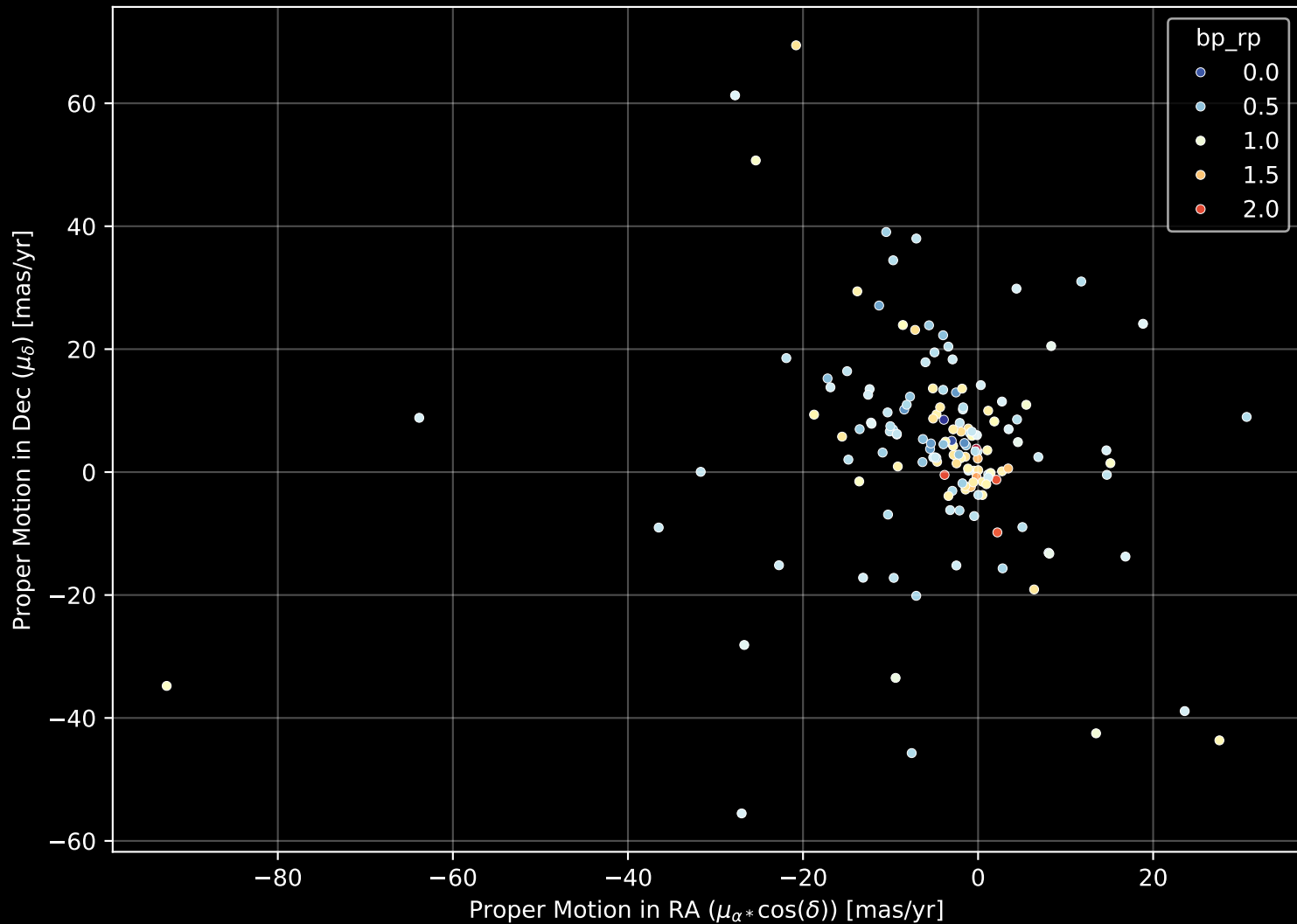
GALAH DR4 Field: [3728] Proper Motion Diagram (n= 150)
