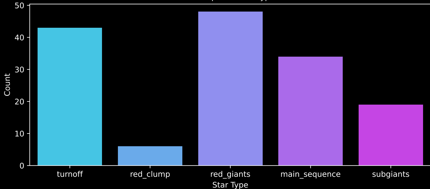
GALAH DR4 Field: [3728] Count plot of Star Type
