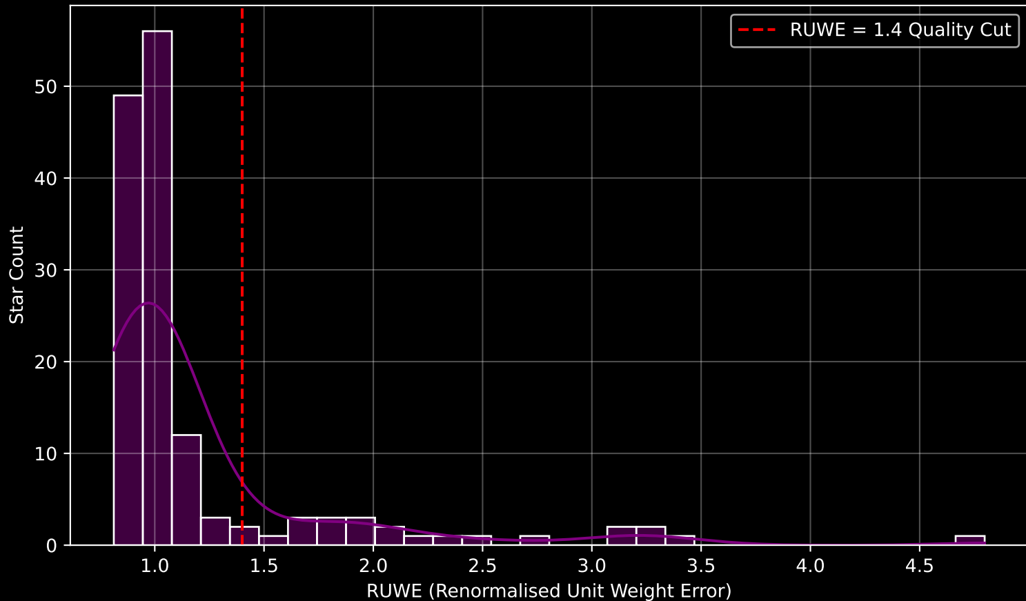
GALAH DR4 Field [3728] RUWE Distribution (n= 144)
